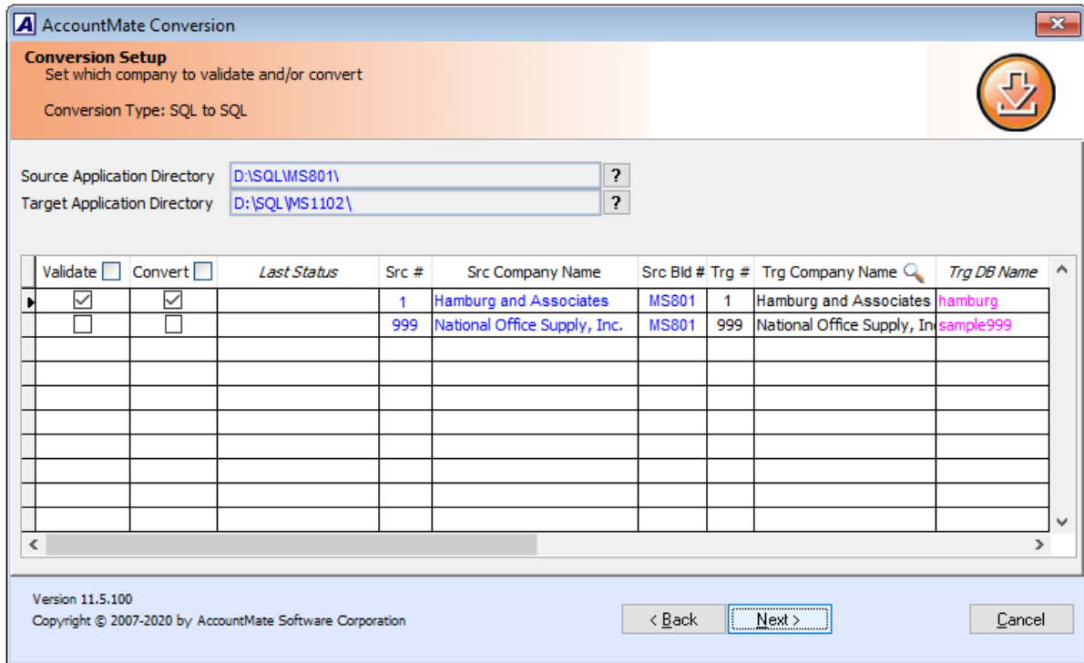
Figure 5. Conversion Setup
