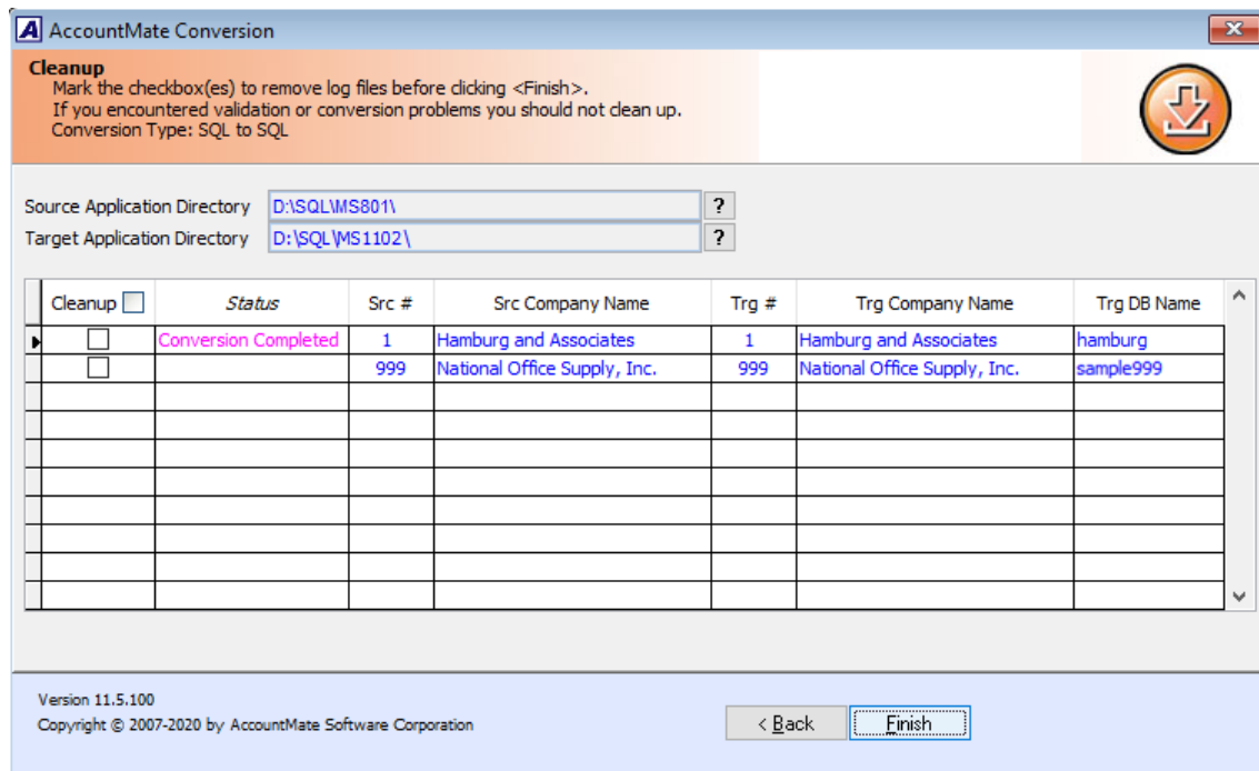
Figure 14. Cleanup Window
