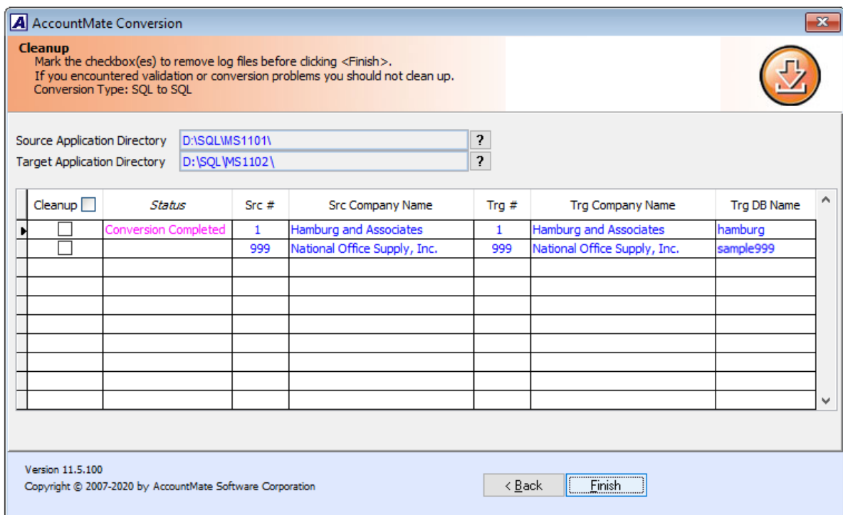
Figure 14. Cleanup Screen
