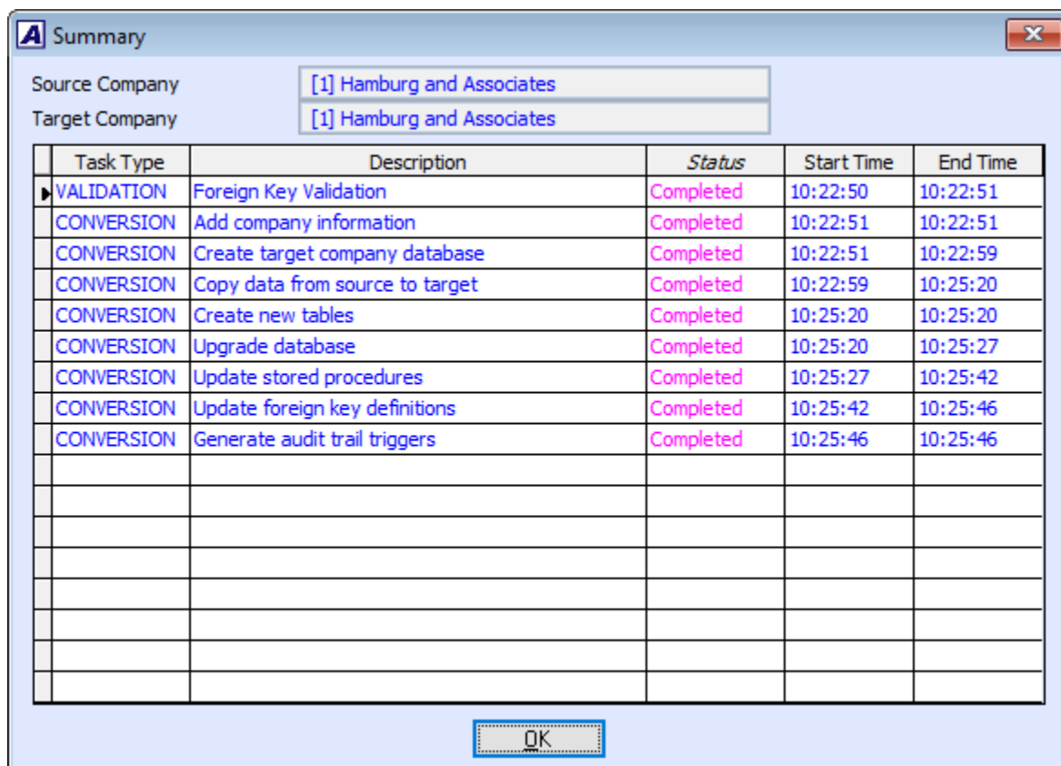
Figure 7b. Summary
