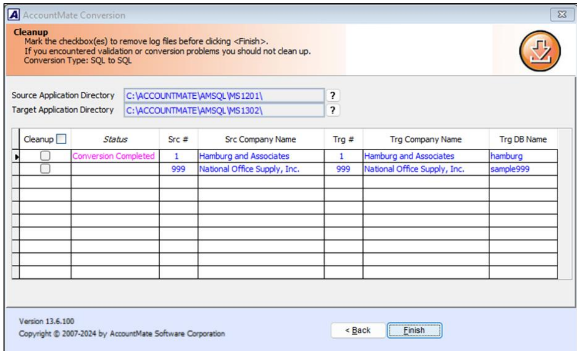
Figure 14. Cleanup Screen
