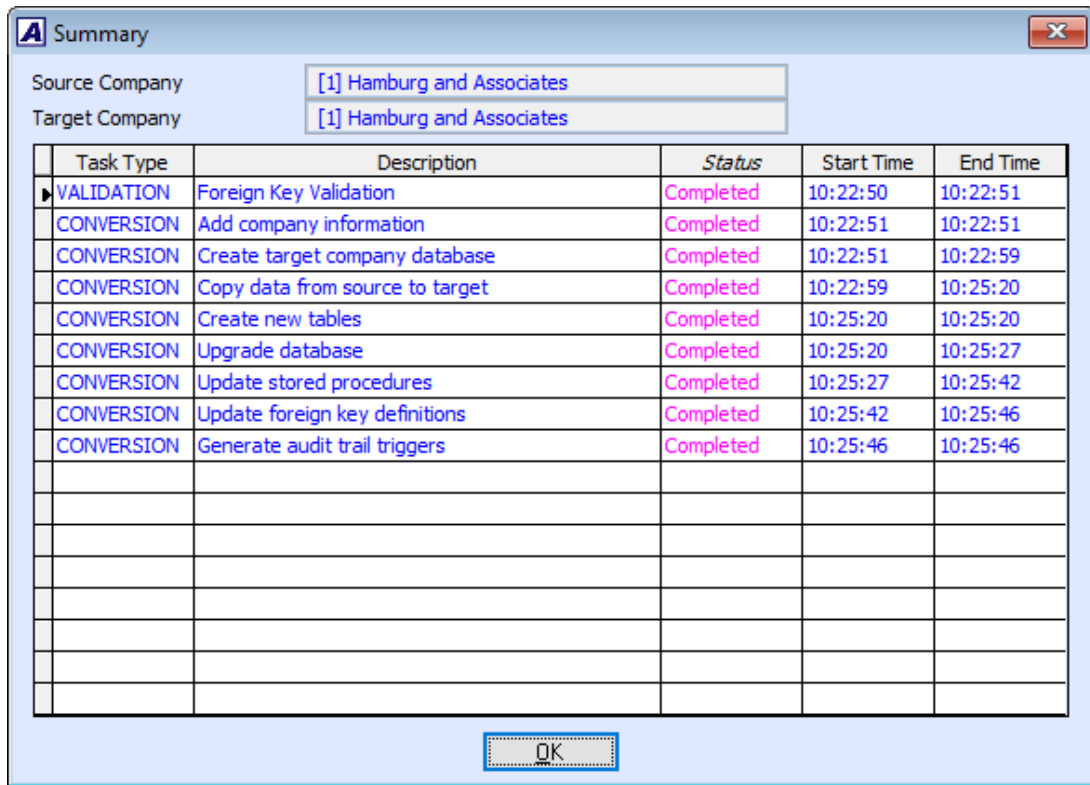
Figure 7b. Summary
