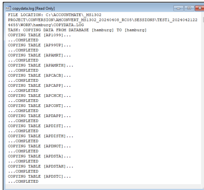
Figure 7c. Upgrade Log
