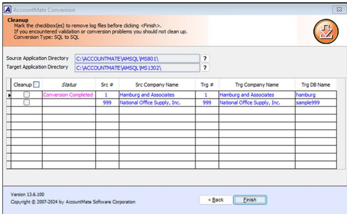
Figure 14. Cleanup Window
