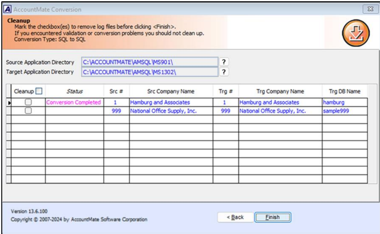
Figure 14. Cleanup Screen
