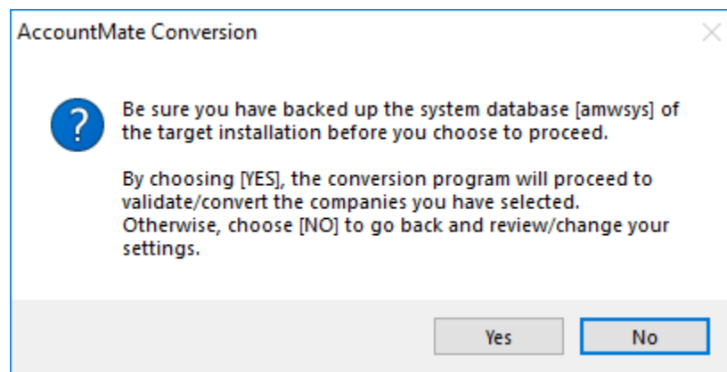
Figure 11. Backup Reminder
