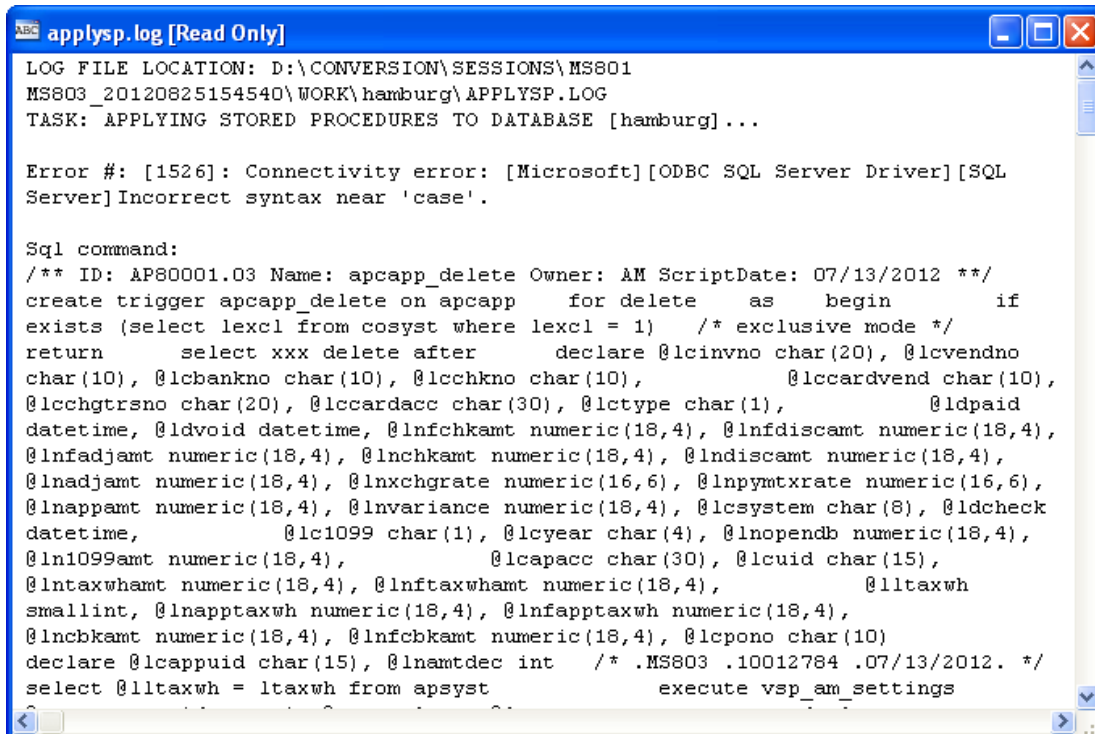
Figure 7c. Update Log
