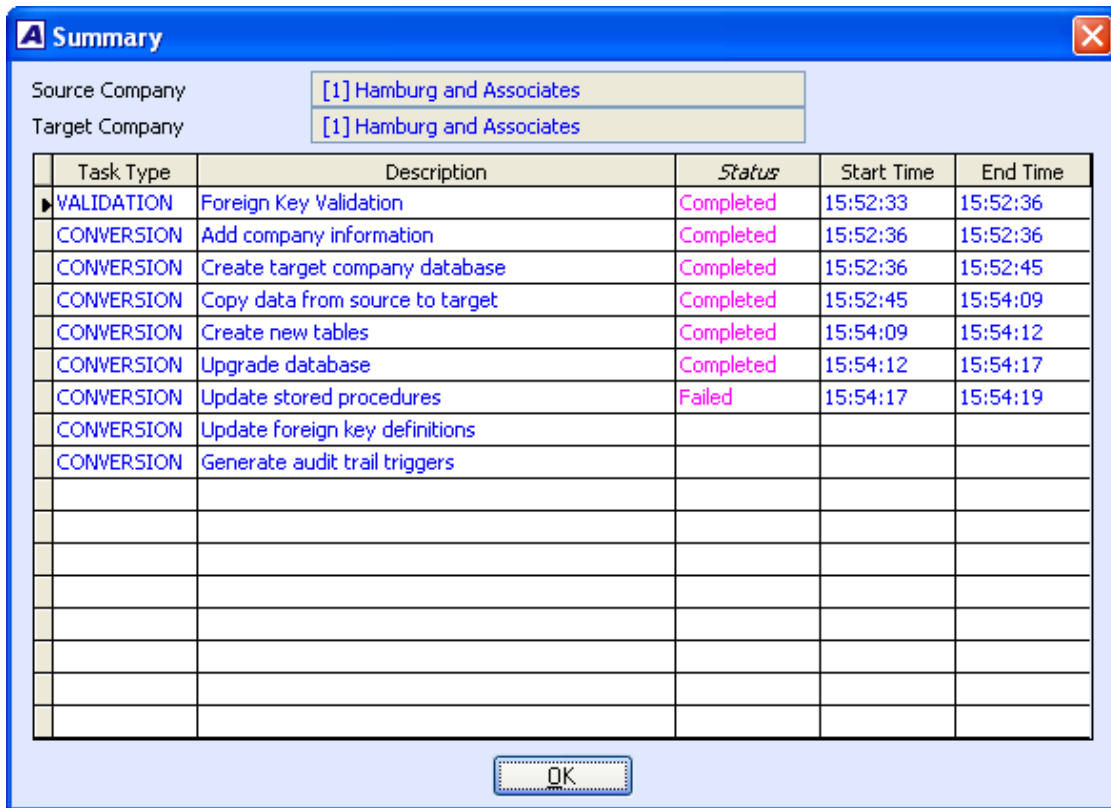
Figure 7b. Summary
