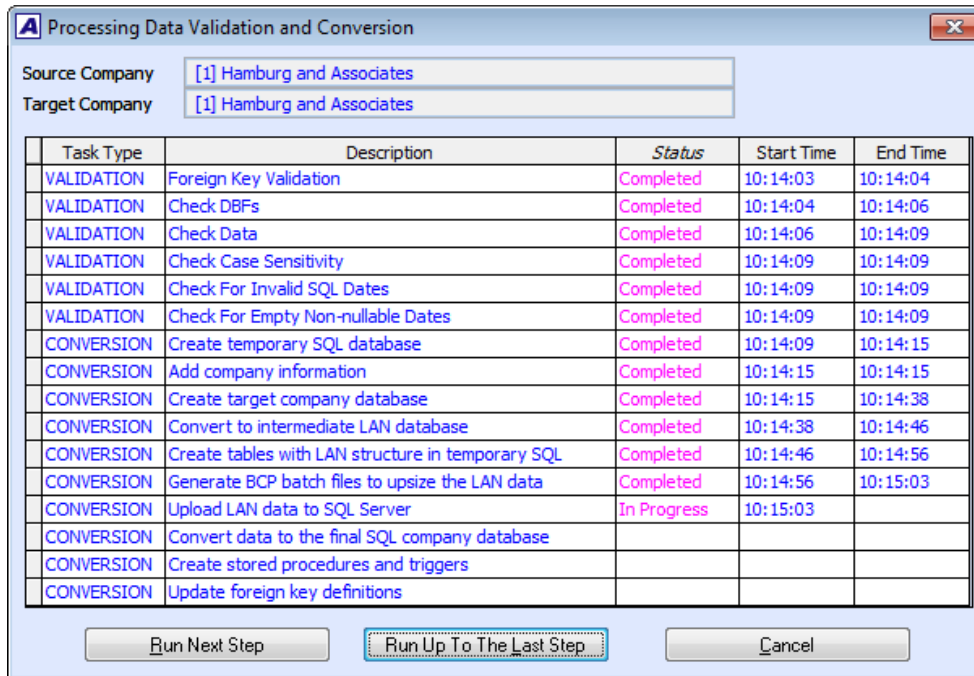
Figure 12. Manual Conversion Process
