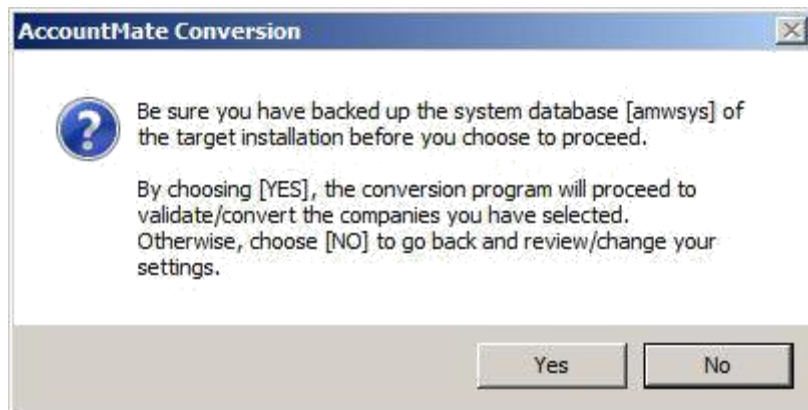
Figure 11. Backup Reminder
