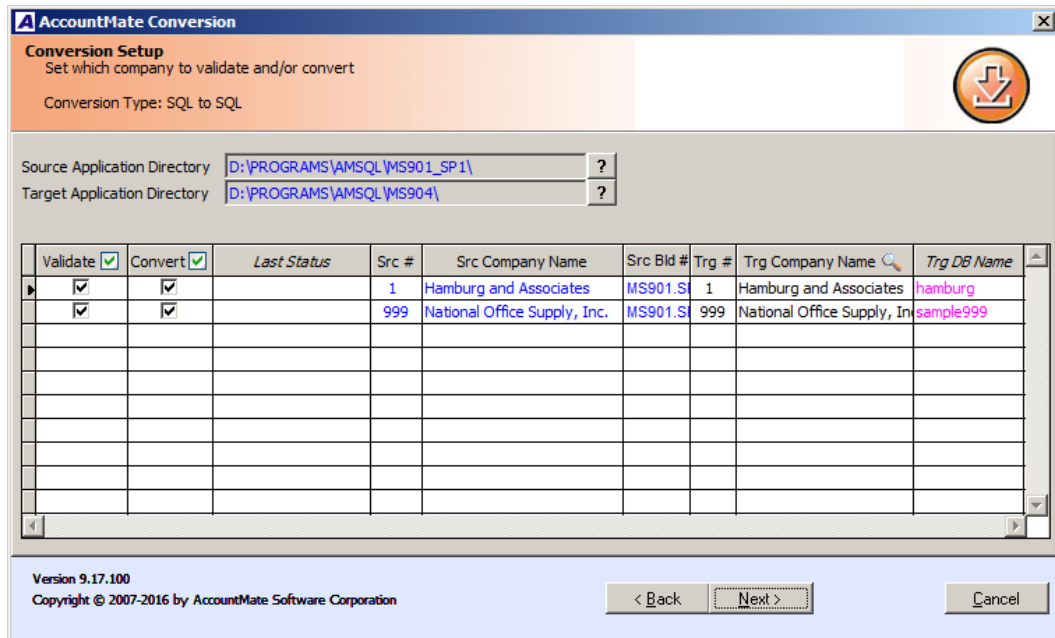
Figure 5. Conversion Setup
