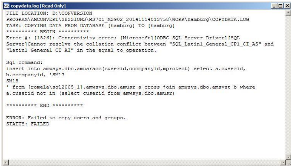
Figure 7c. Upgrade Log
