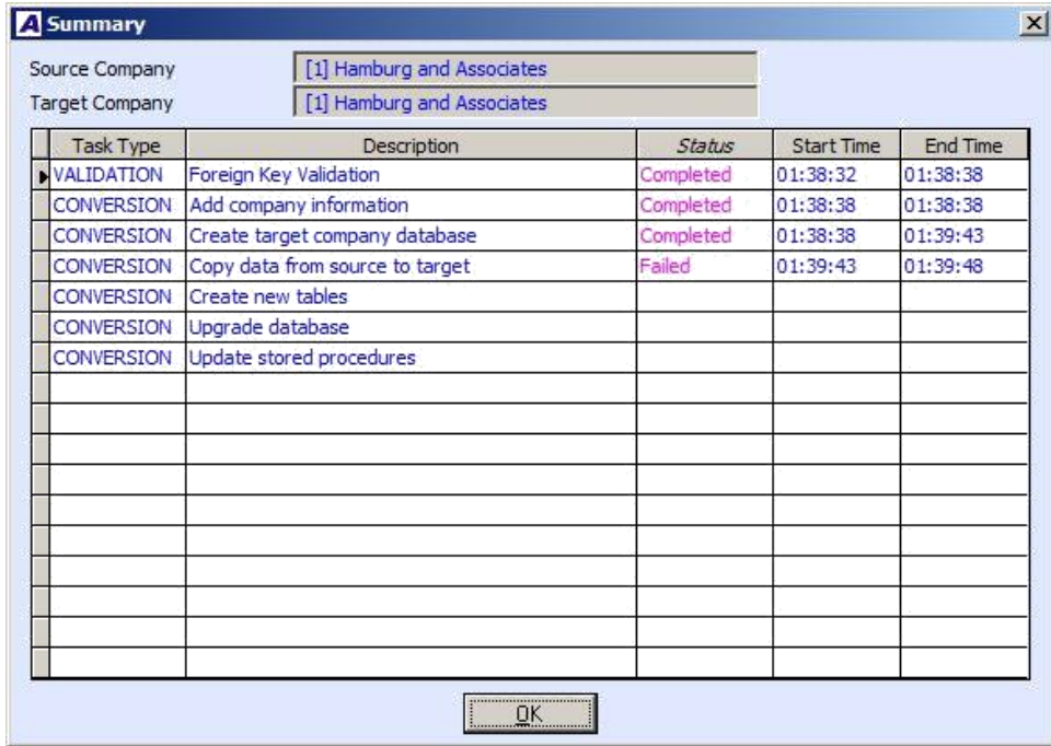
Figure 7b. Summary
